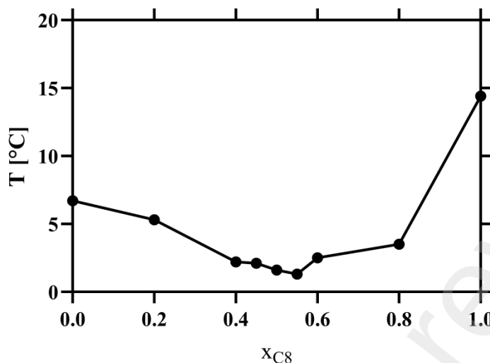
Figure 3. Solid-liquid phase diagram of the binary system C 8 + C 9 fatty acids. x_{C8} – mass fraction of
